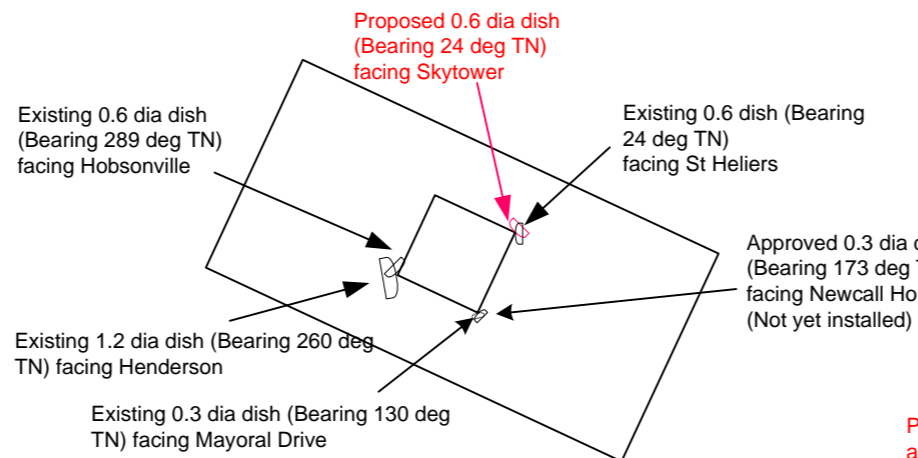
DETAIL 1
