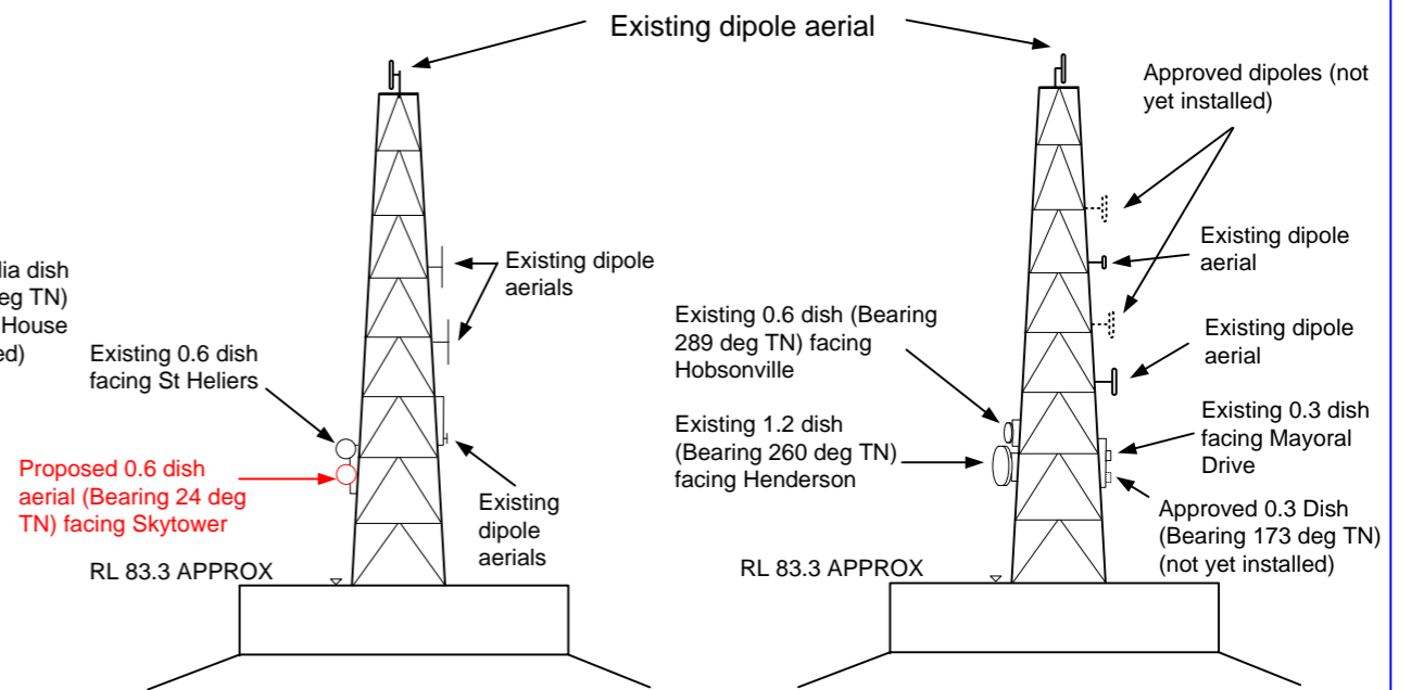
DETAIL 2 1:250
